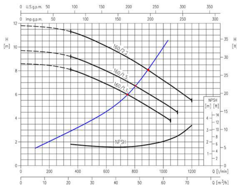
Figure 5. Head-discharge curve of the system and pump and determining the working point of the pumping system.
