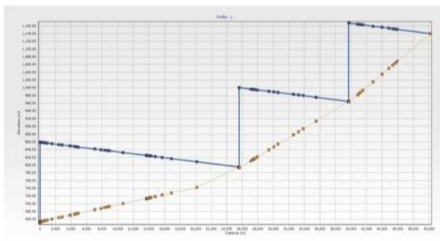
Figure 6. Hydraulic profile of the route with 3 pumping stations (diameter 500 mm).
