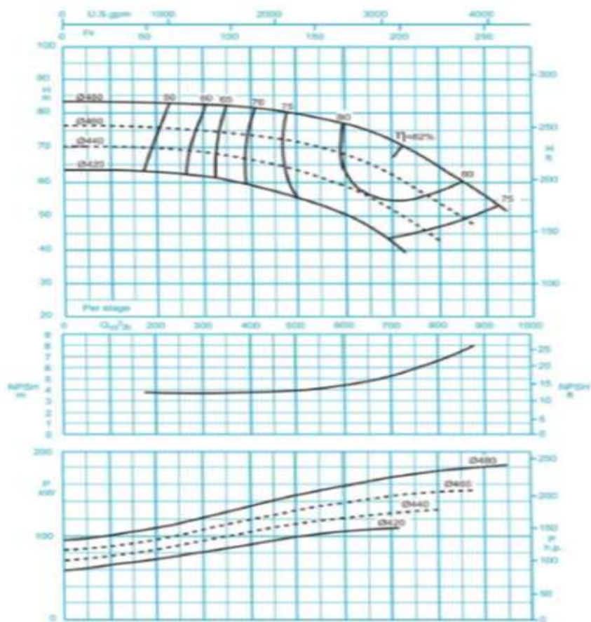
Figure 4. Sample characteristic curve of centrifugal pumps.
