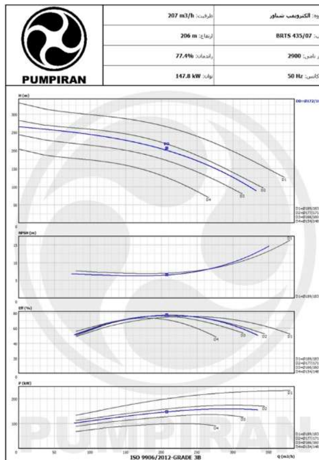
Figure 8. Characteristic curve of deep well submersible centrifugal pump (BRTS/435/07/DD172-166/2900rpm).
