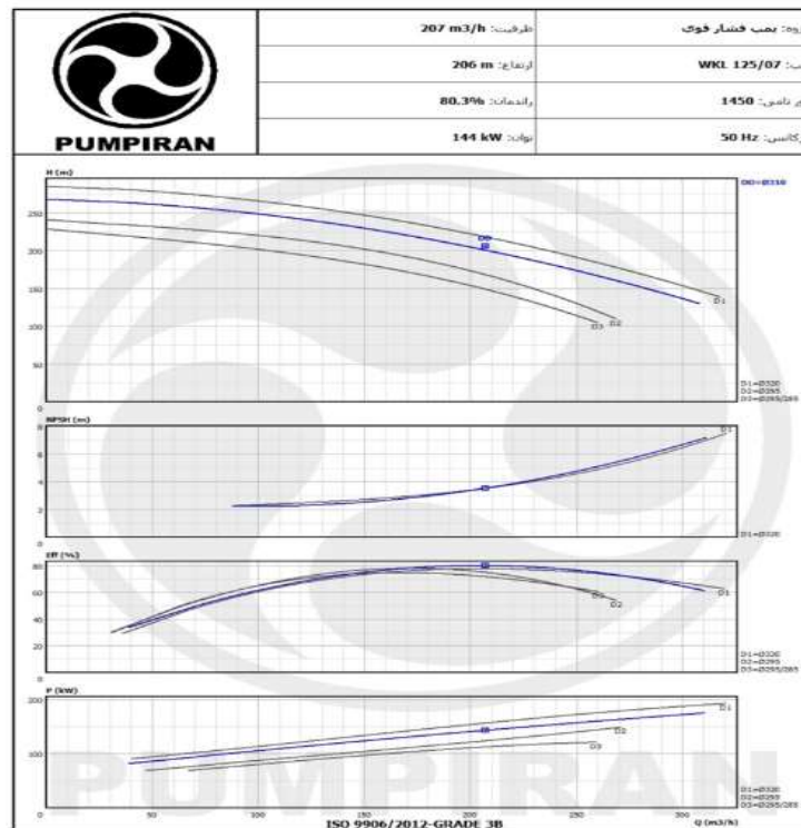
Figure 7. Characteristic curve of horizontal high pressure centrifugal pump (WKL/125/03/DD310/1450rpm)
